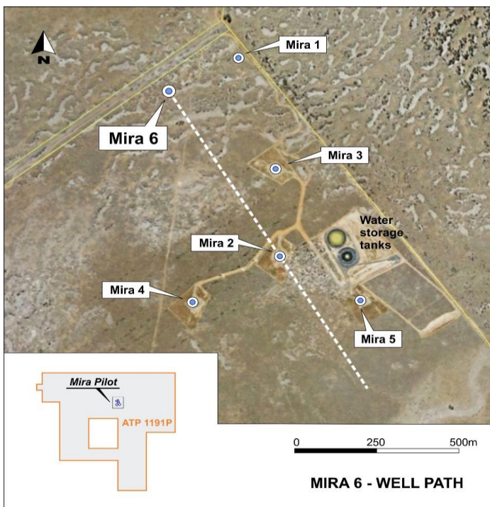
Figure 1 – Mira 6 planned well path
