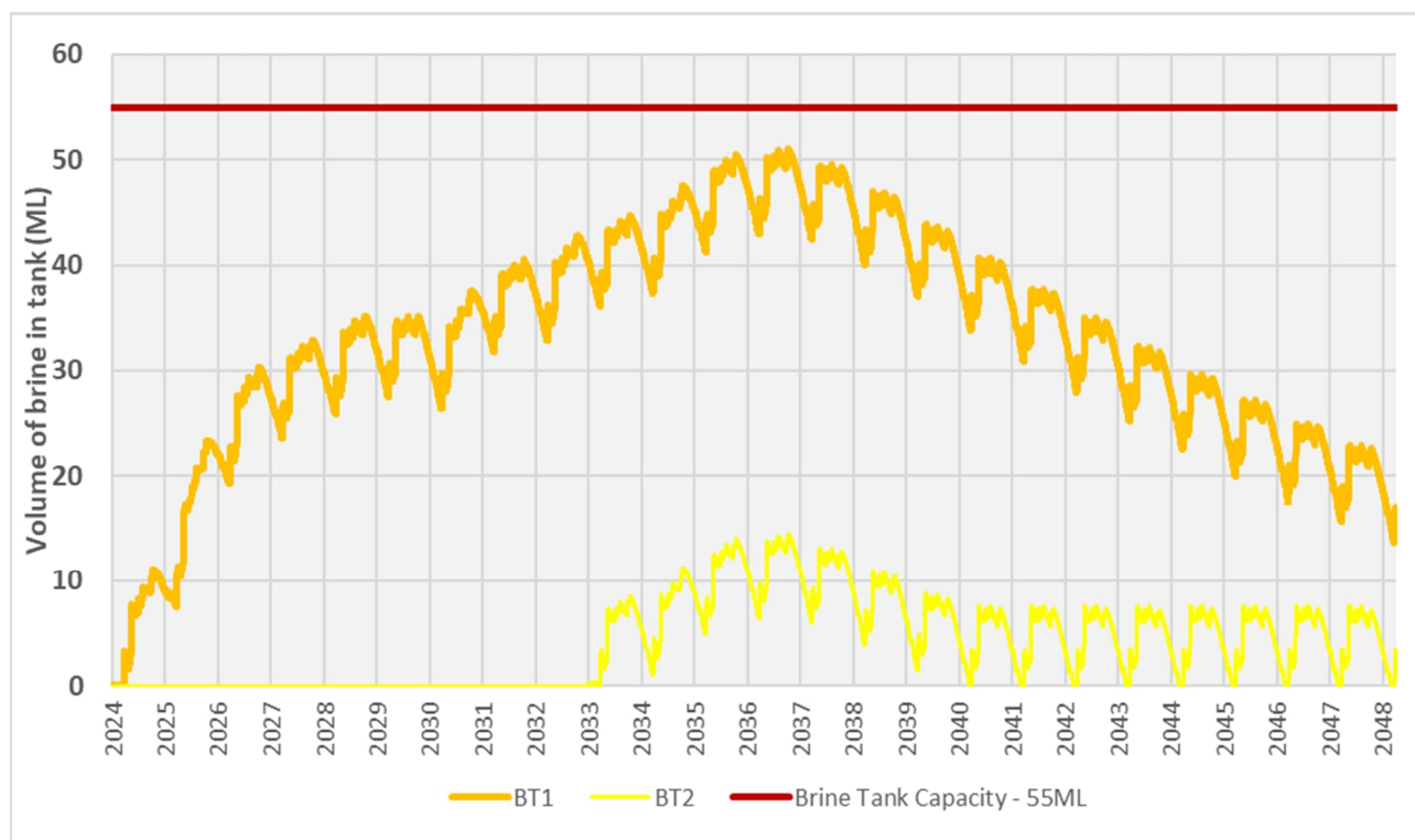
Figure 11 Brine tank volumes – P90 rainfall scenario
