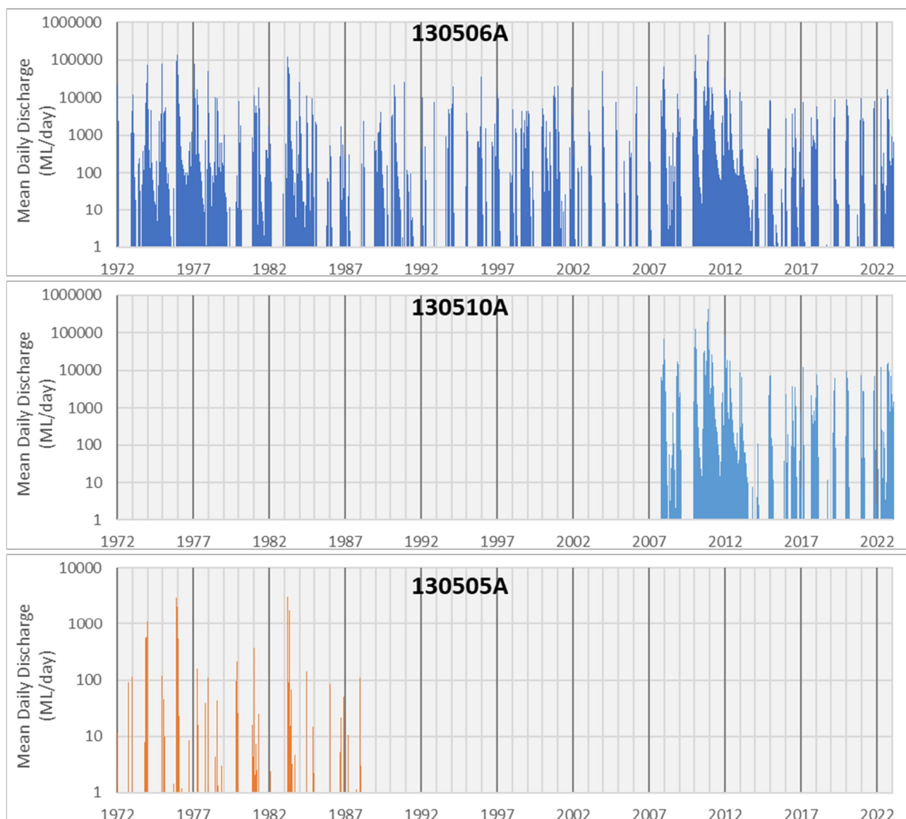
Figure 7 Mean daily discharge at gauging stations
