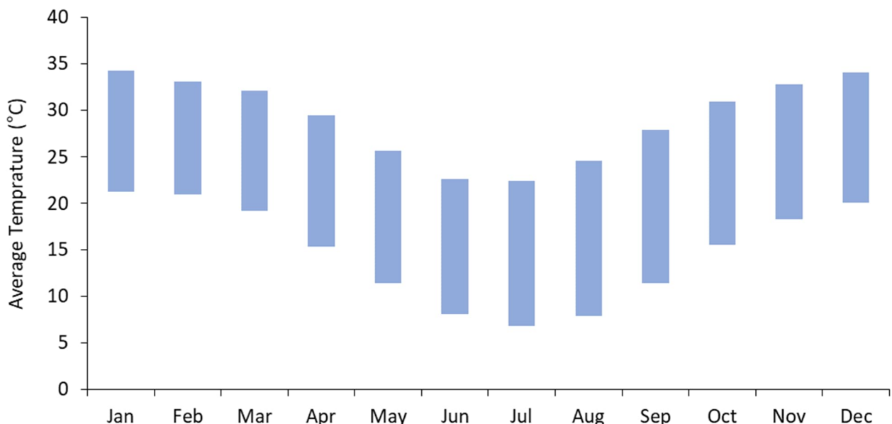
Figure 3 Daily average minimum and maximum temperatures
