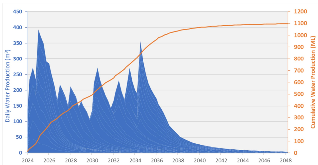
Figure 2 Project water production forecast (April 2023)
