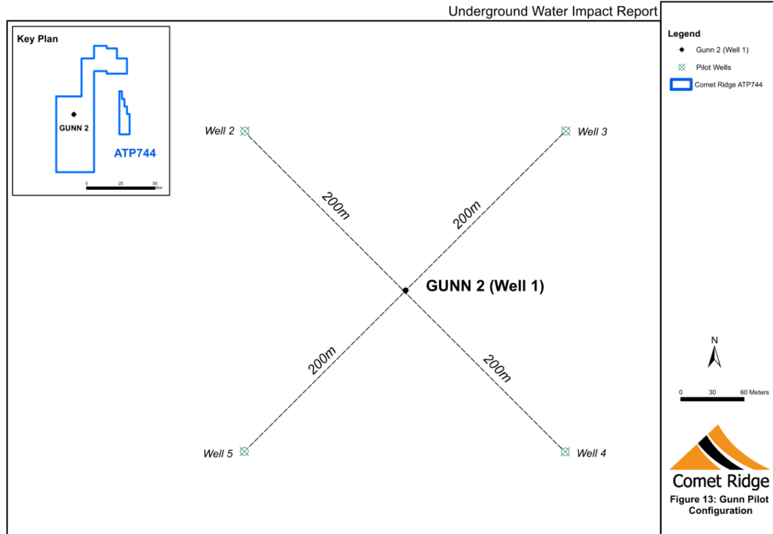
Figure 13: Gunn Pilot Configuration for modelling purposes
